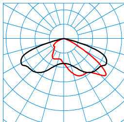
9711SG-AB7L-LRA/51/62/75-740 8G2 (6200 lm) TX064288 ■ C0 - C180 ■ C90 - C270 DIN 5040: A30 UTE: 1,00 H CEN Flux Code: 35 74 98 100 100
