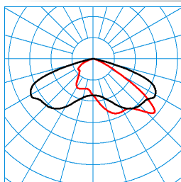
9711SG-AB7L-LRA/51/62/75-740 8G2 (5100 lm) TX064287 ■ C0 - C180 ■ C90 - C270 DIN 5040: A30 UTE: 1,00 H CEN Flux Code: 35 74 98 100 100
