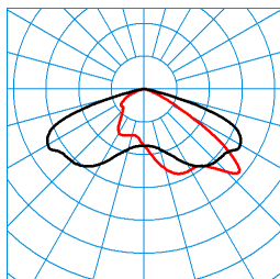
9711SG-AB7L-LRA/51/62/75-740 8G2 (7500 lm) TX064289 ■ C0 - C180 ■ C90 - C270 DIN 5040: A30 UTE: 1,00 H CEN Flux Code: 35 74 98 100 100
