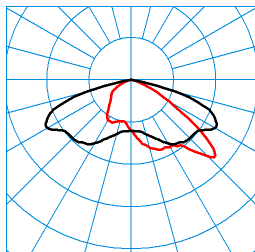
LnPlus 40-AB7L/6200-727 12G1 ETDD (CLO initial value) TX377376 ■ C0 - C180 ■ C90 - C270 DIN 5040: A30 UTE: 1,00 G CEN Flux Code: 35 73 98 100 100
