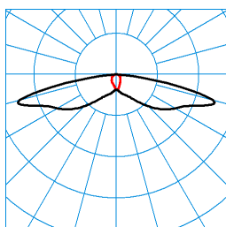
Jovie 50-SB3L-LRA/1000-730 2G1 ET (CLO initial value) TX301042 ■ C0 - C180 ■ C90 - C270 DIN 5040: A20 UTE: 1,00 l CEN Flux Code: 29 61 91 100 100
