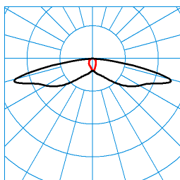
Jovie 50-SB3L-LRA/1000-730 2G1 ET (CLO end value) TX300874 ■ C0 - C180 ■ C90 - C270 DIN 5040: A20 UTE: 1,00 l CEN Flux Code: 29 61 91 100 100
