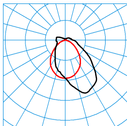
TugraHE 12 PAW 23-71/16ML-830 ET PC 23 (STAG12) TX425184 ■ C0 - C180 ■ C90 - C270 DIN 5040: B40 UTE: 0,86 E + 0,14 T CEN Flux Code: 48 77 92 86 100 13 32 64 14
