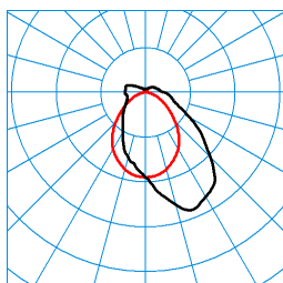
TugraHE 12 PAW 23-71/16ML-830 ET PC 23 (STAG14) TX425231 ■ C0 - C180 ■ C90 - C270 DIN 5040: B40 UTE: 0,86 E + 0,14 T CEN Flux Code: 48 77 92 86 100 13 32 64 14
