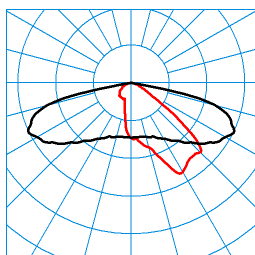
LIQ 50N-AB2L-LR/2600-727 4G1 ET (CLO initial value) TX278078 ■ C0 - C180 ■ C90 - C270 DIN 5040: A30 UTE: 1,00 G CEN Flux Code: 34 71 96 100 100 0 0 0 0
