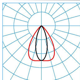
ELINE FL LVN160 865 L225 1 20
