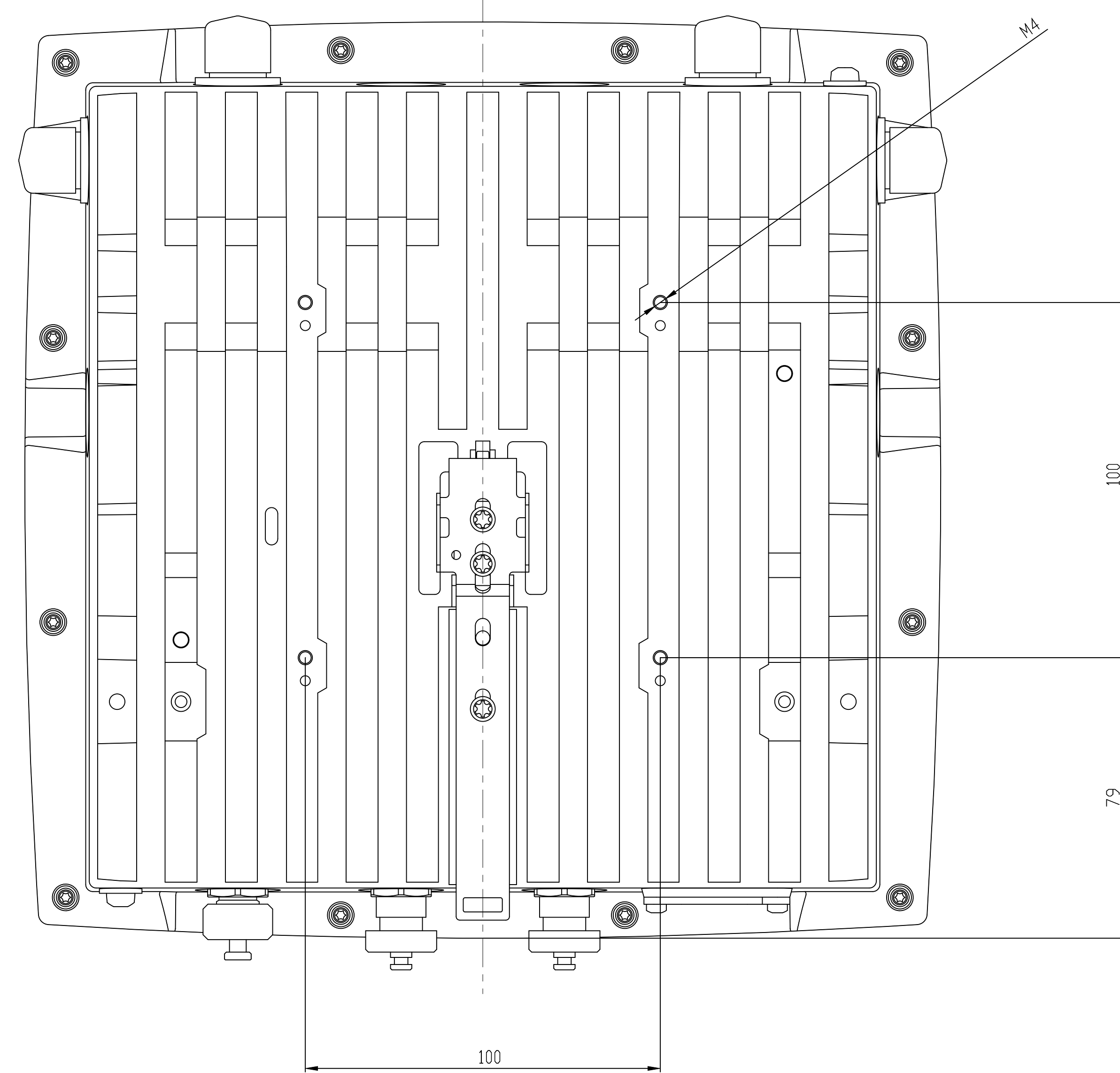
Drilling
