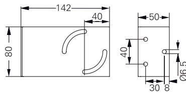
Mounting bracket
