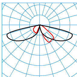
CS 19 100-AB2L/1650-730 2G1S ETDD (CLO initial value) TX299967 ■ C0 - C180 ■ C90 - C270 DIN 5040: A20 UTE: 1,00 l CEN Flux Code: 26 63 96 100 100
