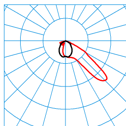
Jovie 50I-AM2L-SLR1/4200-730 4G1 ET (CLO end value) TX301451 ■ C0 - C180 ■ C90 - C270 DIN 5040: A40 UTE: 1,00 F CEN Flux Code: 47 91 100 100 100
