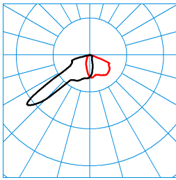
Jovie 70-FL1L/6800-730 8G1 ET (CLO initial value) TX300558 ■ C0 - C180 ■ C90 - C270 DIN 5040: A40 UTE: 1,00 F CEN Flux Code: 38 80 98 100 100
