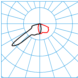
Jovie 70-FL1L/6800-730 8G1 ET (CLO end value) TX300510 ■ C0 - C180 ■ C90 - C270 DIN 5040: A40 UTE: 1,00 F CEN Flux Code: 38 80 98 100 100
