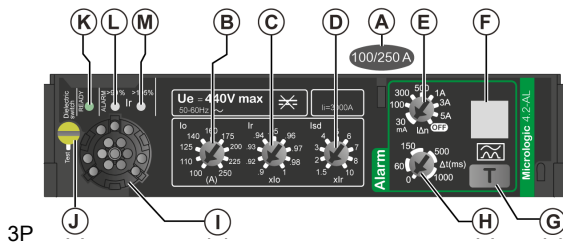
Version Alarme Micrologic 4.2AL
