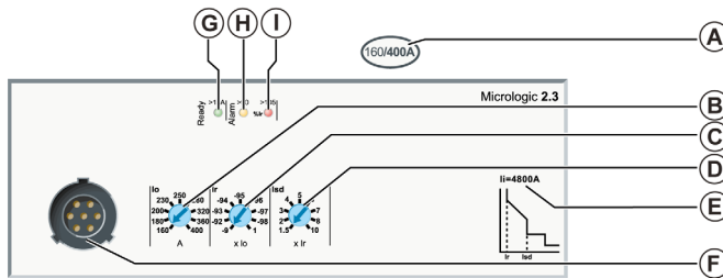
Version Micrologic 2.3 3P
