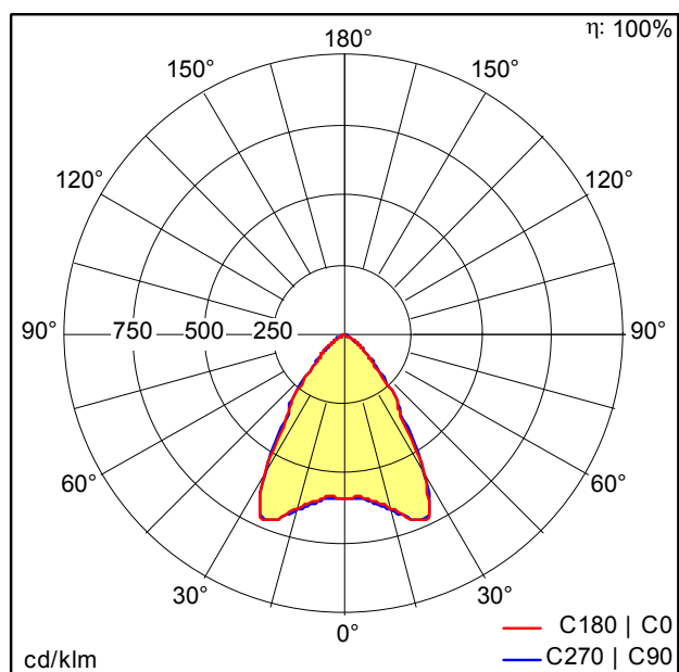
D38477AA_TECTON_MIREL_LED4000-840_L1500_EVG.IDT
