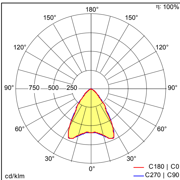
D38477AA_TECTON_MIREL_LED5400-840_L2000_EVG.idt
