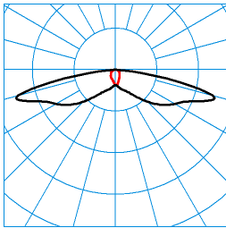
Jovie 50-SB3L-LR/1000-740 2G1 ET (CLO end value) TX301143 ■ C0 - C180 ■ C90 - C270 DIN 5040: A20 UTE: 1,00 l CEN Flux Code: 29 61 91 100 100
