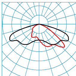
Jovie 70-AB7L-ML/5600-6800-730 8G1 ETDD (CLO end value) TX271460 ■ C0 - C180 ■ C90 - C270 DIN 5040: A30 UTE: 1,00 G CEN Flux Code: 34 71 96 100 100
