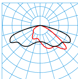
Jovie 70-AB7L-ML/5600-6800-730 8G1 ETDD (CLO initial value) TX271459 ■ C0 - C180 ■ C90 - C270 DIN 5040: A30 UTE: 1,00 G CEN Flux Code: 34 71 96 100 100
