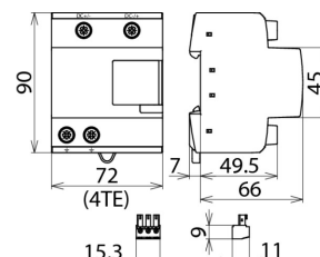
Dimensions DCB YPV 1200 FM
