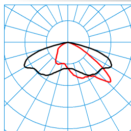
LnPlus 40-AB7L-LR/2200-730 2G1 ET (CLO end value) TX377119 DIN 5040: A30 UTE: 1,00 G CEN Flux Code: 35 73 98 100 100
