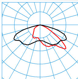
LnPlus 40-AB7L/6200-722 12G1 ETDD (CLO end value) TX377592 ■ C0 - C180 ■ C90 - C270 DIN 5040: A30 UTE: 1,00 G CEN Flux Code: 35 73 98 100 100
