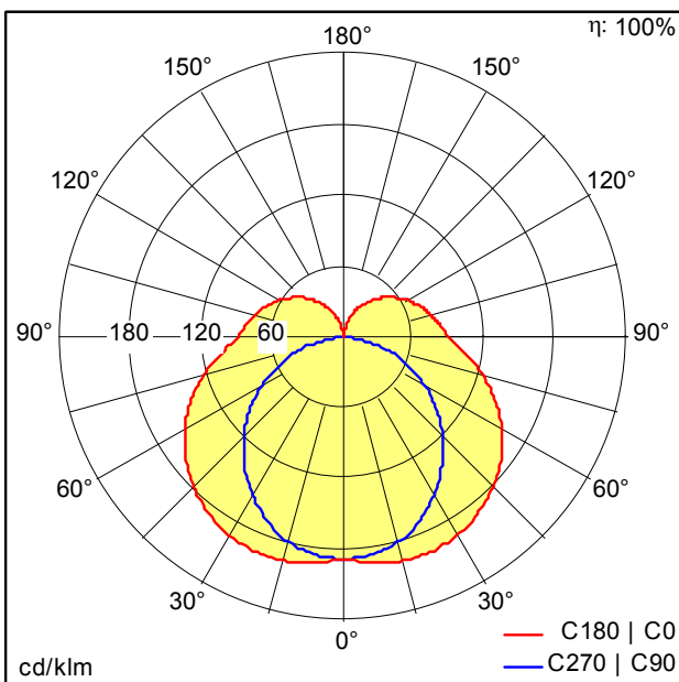
D39718AA_LINARIA_LED2200-840_L908_PM_SR.Idt
