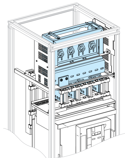
Okken switchboard
