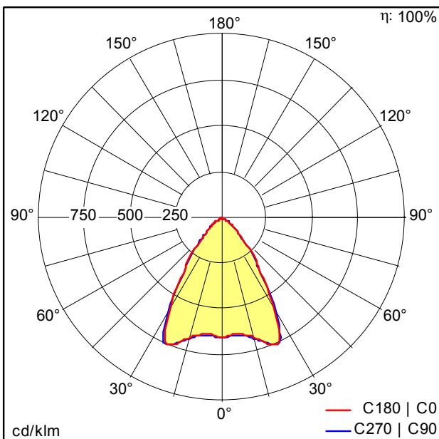
D42326AA_TECTON_MIRL_LED3700-840_L1000_LDO_BK.Idt
