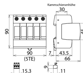
Dimensions DG M PV2 SCI 1000 FM
