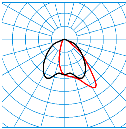
Jovie 70I-AM3L/10000-730 8G1 ETDD (CLO initial value) TX301052 ■ C0 - C180 ■ C90 - C270 DIN 5040: A50 UTE: 1,00 D CEN Flux Code: 59 89 100 100 100
