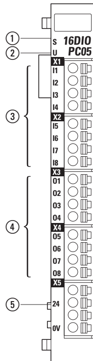
Figure 71: XN-322-16DIO-PC05 LEDs
