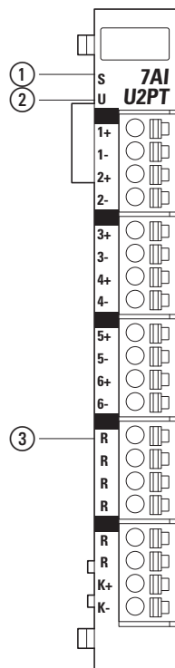
Figure 82: LED signals and pin assignment
