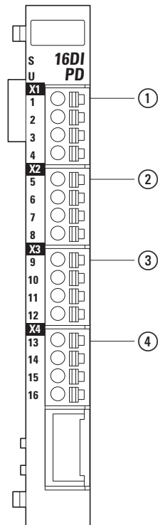
Figure 27: Pin assignment
