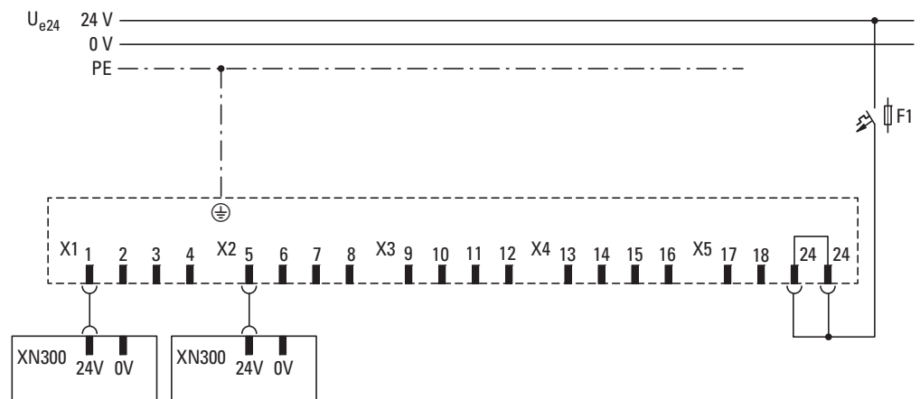
Figure 21: Wiring example
