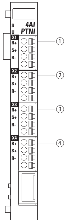
Figure 78: Pin assignment
