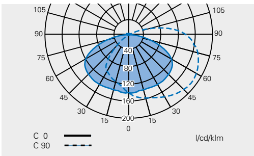
Polar curve NVMV 70 - 250 W (with external reflector RA 70)
