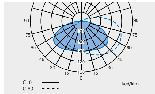
Polar curve NVMV 250 - 400 W (with external reflector RA 739)
