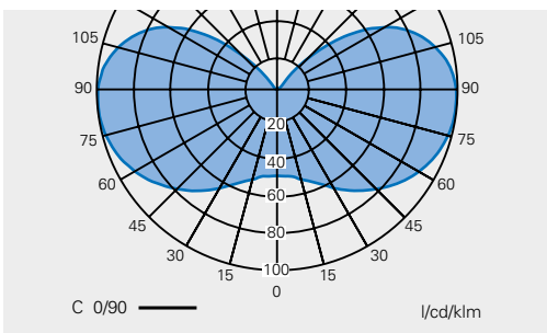
Polar curve NVMV 70 - 250 W (without external reflector)
