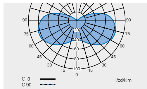
Polar curve NVMV 250 - 400 W (without external reflector)
