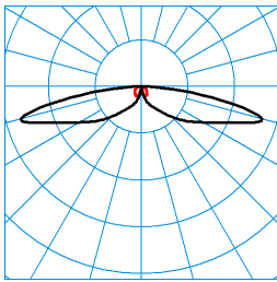
CS 19 100-SB3L-SLR1/5100-730 4G1S ET (CLO end value) TX300159 ■ C0 - C180 ■ C90 - C270 DIN 5040: A20 UTE: 1,00 J CEN Flux Code: 23 53 85 100 100 0 0 0 0
