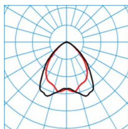
ELINE LW40-110 ML 830 L150 2 50
