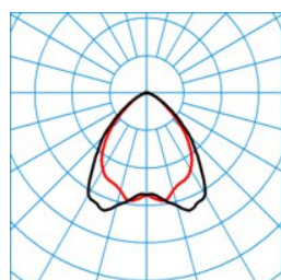
ELINE LW40-110 ML 830 L150 0 50
