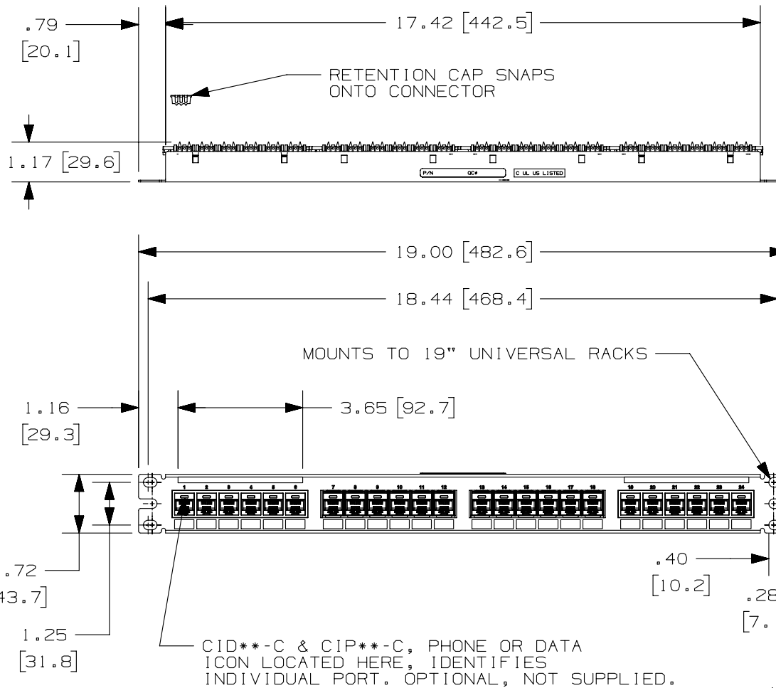
FIGURE 1 DP6 PLUS 24 PORT PATCH PANEL
