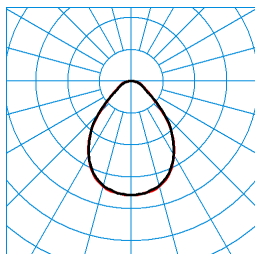
ArimoFit M48 PW19 53-840 ET + ArimoFit Sky M48-TS ZER TX426324 ■ C0 - C180 ■ C90 - C270 UGR I = 17,7 UGR q = 17,7 DIN 5040: A50 UTE: 1,00 C CEN Flux Code: 65 89 97 100 100 0 0 0 0
