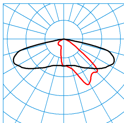
Jovie 50-AB2L-ML/1000-2200-740 2G1 ETDD (CLO end value) TX271465 ■ C0 - C180 ■ C90 - C270 DIN 5040: A30 UTE: 0,98 l CEN Flux Code: 34 70 96 100 98
