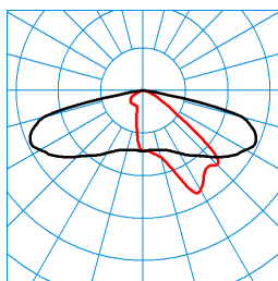
Jovie 50-AB2L-ML/1000-2200-740 2G1 ETDD (CLO initial value) TX271556 ■ C0 - C180 ■ C90 - C270 DIN 5040: A30 UTE: 0,98 l CEN Flux Code: 34 70 96 100 98
