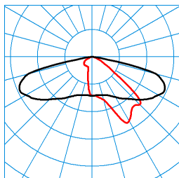
Jovie 50-AB2L-ML/1000-2200-740 2G1 ETDD (2200 lm) TX068680 ■ C0 - C180 ■ C90 - C270 DIN 5040: A30 UTE: 0,98 l CEN Flux Code: 34 70 96 100 98
