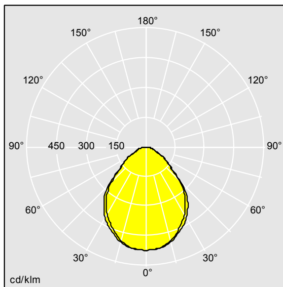
D44261AA_EQL_840_HF_L1500_LRO_WH_.ldt
