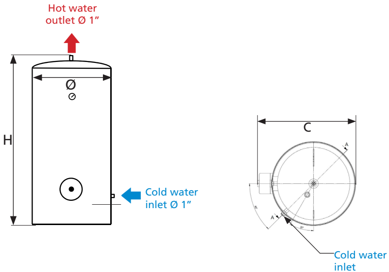
Schematic view
