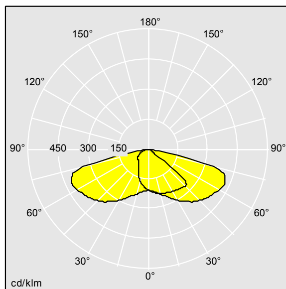
TL_IP60L35NR730.ltd
