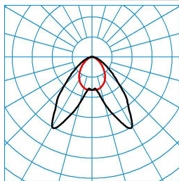
ELINE LDAH100 840 L225 1 20
