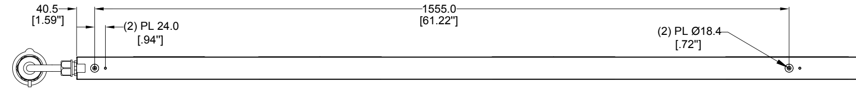
REAR VIEW
