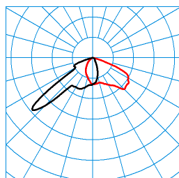
LIQ 50N-FL1L/4200-730 4G1 ET (CLO initial value) TX278070 ■ C0 - C180 ■ C90 - C270 DIN 5040: A40 UTE: 1,00 F CEN Flux Code: 43 84 100 100 100
