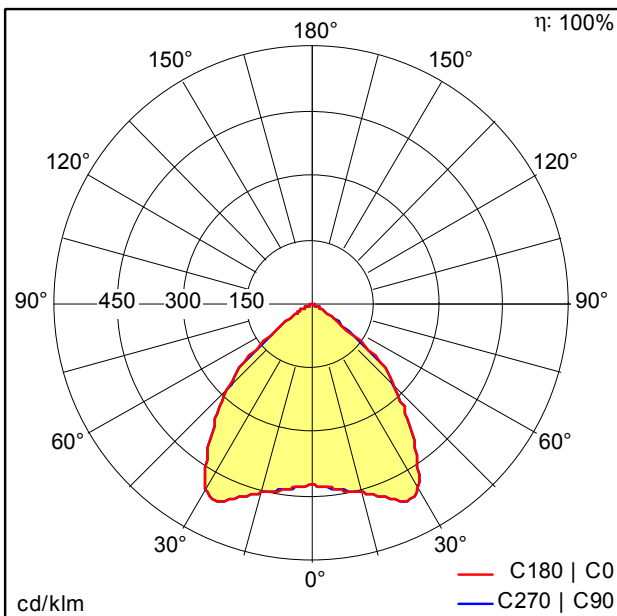
D43022_MIRL_NIV_2800-830_M600Q_WB_EVG_WH.Idt
