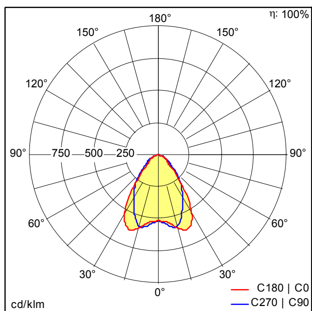
D35001AA_TECTON_C_LED7400-830_L2000_WB_LDE_WH.Idt
