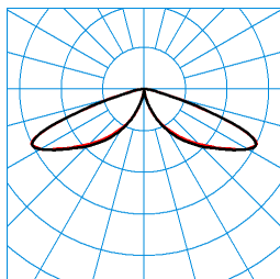
LTX LT-RB6L-LRA/15/18/26-740 4G1 (2600 lm) TX084122 ■ C0 - C180 ■ C90 - C270 DIN 5040: A20 UTE: 1,00 J CEN Flux Code: 15 51 96 100 100 0 0 0 0
