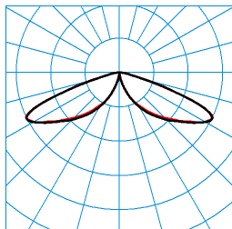
LTX LT-RB6L-LRA/15/18/26-740 4G1 (1800 lm) TX084121 ■ C0 - C180 ■ C90 - C270 DIN 5040: A20 UTE: 1,00 J CEN Flux Code: 15 51 96 100 100 0 0 0 0
