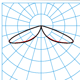
LTX LT-RB6L-LRA/15/18/26-740 4G1 (1500 lm) TX084120 ■ C0 - C180 ■ C90 - C270 DIN 5040: A20 UTE: 1,00 J CEN Flux Code: 15 51 95 100 100 0 0 0 0
