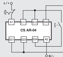
Input configuration with manual start 1 channel
