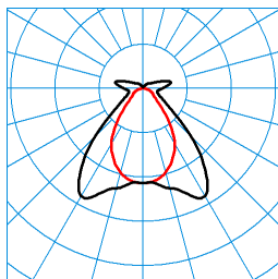
TugraHE Act 12 PW19 34 ETDD8 01 (ACTDSU) TX375184 C0 - C180 C90 - C270 DIN 5040: B41 UTE: 0,81 D + 0,19 T CEN Flux Code: 60 85 94 81 100 9 28 64 19
