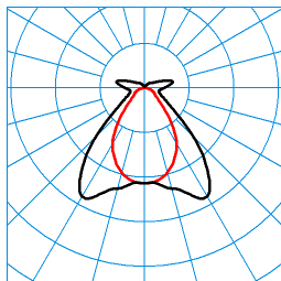
TugraHE Act 12 PW19 34 ETDD8 01 (ACTDCW) TX375183 C0 - C180 C90 - C270 DIN 5040: B41 UTE: 0,81 D + 0,19 T CEN Flux Code: 60 85 94 81 100 9 28 64 19
