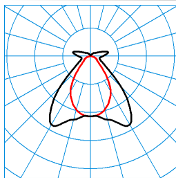
TugraHE Act 12 PW19 34 ETDD8 01 (ACTDWW) TX375185 C0 - C180 C90 - C270 DIN 5040: B41 UTE: 0,81 D + 0,19 T CEN Flux Code: 60 85 94 81 100 9 28 64 19
