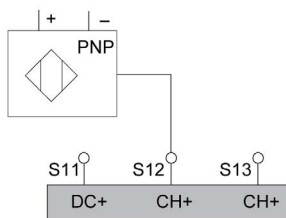
Wiring of the inputs for sensors/devices with PNP output
