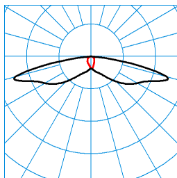
Jovie 50-SB3L-LRA/1000-740 2G1 ET (CLO initial value) TX300429 ■ C0 - C180 ■ C90 - C270 DIN 5040: A20 UTE: 1,00 l CEN Flux Code: 29 61 91 100 100
