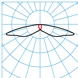
Jovie 50-SB3L-LRA/1000-740 2G1 ET (CLO end value) TX301577 ■ C0 - C180 ■ C90 - C270 DIN 5040: A20 UTE: 1,00 l CEN Flux Code: 29 61 91 100 100
