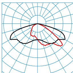
LIQ 70N-AB7L-LR/14500-727 12G1 ET (CLO initial value) TX278217 ■ C0 - C180 ■ C90 - C270 DIN 5040: A30 UTE: 1,00 G CEN Flux Code: 35 73 98 100 100 0 0 0 0
