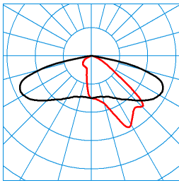
Jovie 50-AB2L-LR/2200-730 4G1 ET (CLO initial value) TX301798 ■ C0 - C180 ■ C90 - C270 DIN 5040: A30 UTE: 1,00 G CEN Flux Code: 34 71 96 100 100
