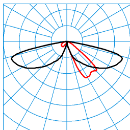
LTX K-AB2L-LRA/15/18/26-730 4G1 (1500 lm) TX059696 ■ C0 - C180 ■ C90 - C270 DIN 5040: A20 UTE: 1,00 l CEN Flux Code: 24 61 92 100 100 0 0 0 0
