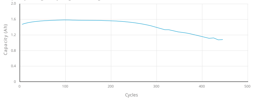
Capacity change in cycling after charge at 1C
