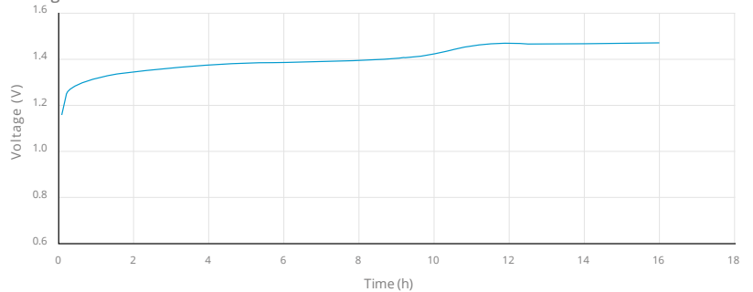
Charge at C/10
