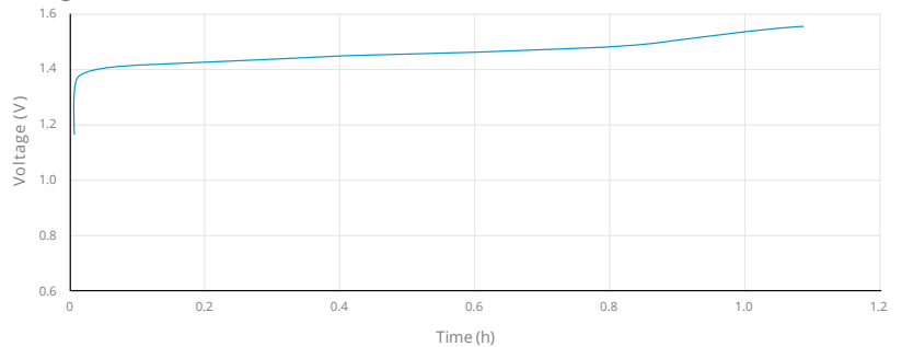
Charge at 1C
