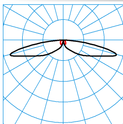
CS 19 100-SB3L-SLR1/5100-740 4G1S ET (CLO end value) TX300161 ■ C0 - C180 ■ C90 - C270 DIN 5040: A20 UTE: 1,00 J CEN Flux Code: 23 53 85 100 100 0 0 0 0
