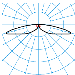
CS 19 100-SB3L-SLR1/5100-740 4G1S ET (CLO initial value) TX300162 ■ C0 - C180 ■ C90 - C270 DIN 5040: A20 UTE: 1,00 J CEN Flux Code: 23 53 85 100 100 0 0 0 0
