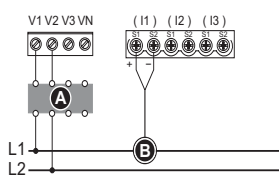
1PH2W L-L
